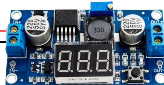
ADJUSTABLE BUCK CONVERTER
